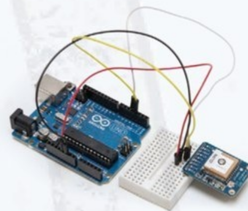
The Adafruit Ultimate GPS Breakout board. A typical GPS interface, assuming both module and main board run at compatible voltages, is as simple as connecting four wires.
