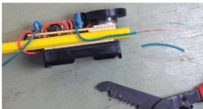
4. Attach the perfboard and battery holder to the pencil.
