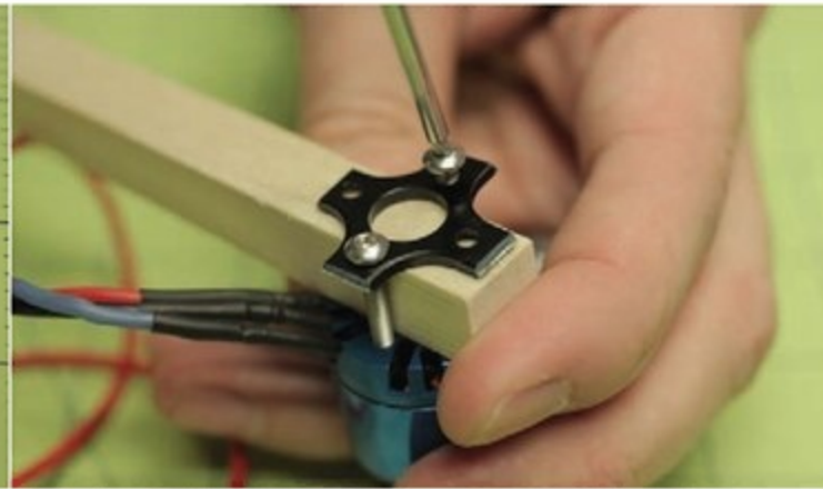
5b Only 2 screws are used on each motor for mounting, and the factory brackets are cut down to save weight.
