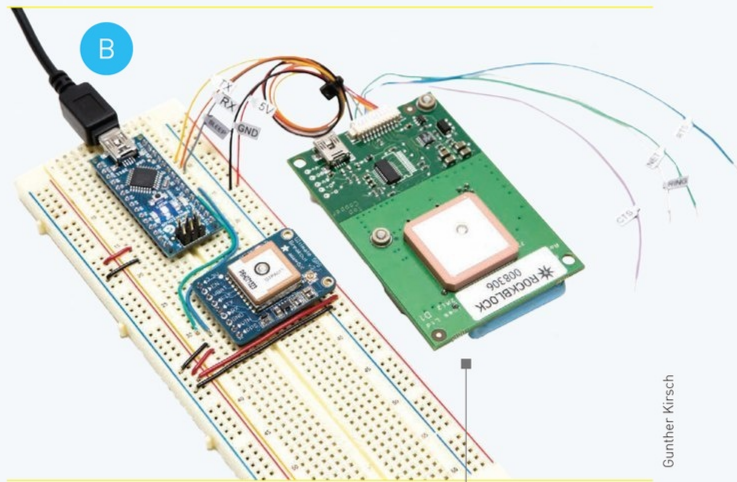
Each RockBlock ships with a 10-pin JST-terminated cable that snaps onto the board and exposes the various signal lines client devices can connect to. The simplest setup, shown here, is what Iridium calls a "3-wire" TTL serial interface, with signal lines for TX, RX, and Sleep. (To connect your Arduino and GPS as shown, see page 59.)
