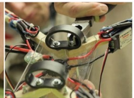
6 The gimbal and battery shelf are attached via 2 shock mounts cut from thick flexible rubber tubing, which helps isolate the camera from propeller vibrations and adds a bit of space, above, to mount the gimbal controller board.
