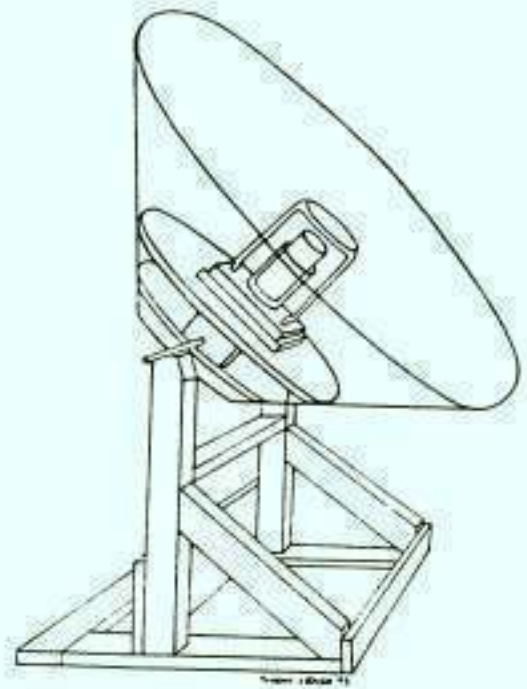
Conical Solar Cooker.
