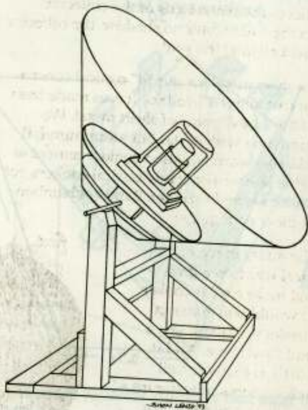
Conical Solar Cooker.
