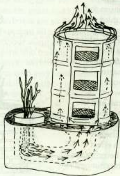
How flue gases pass between the drums.
