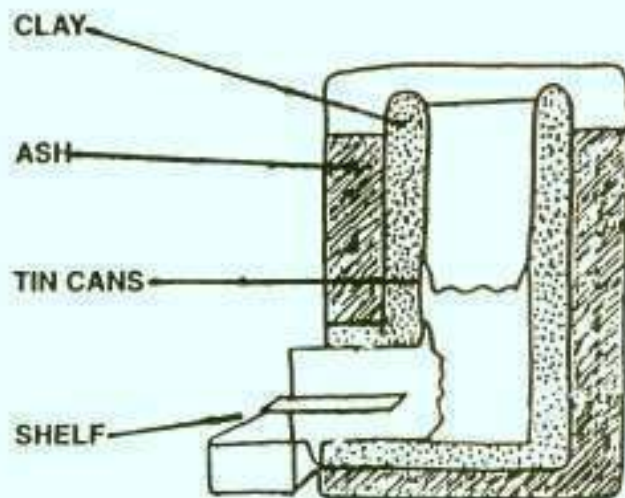
THE STOVE WITH CLAY/SAND AROUND THE TIN CANS
