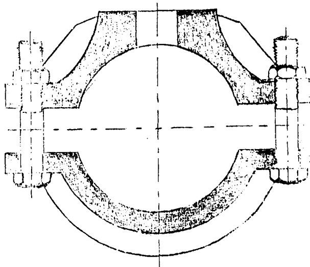
(viii) Saddle Piece (F/F/F) Cross section
